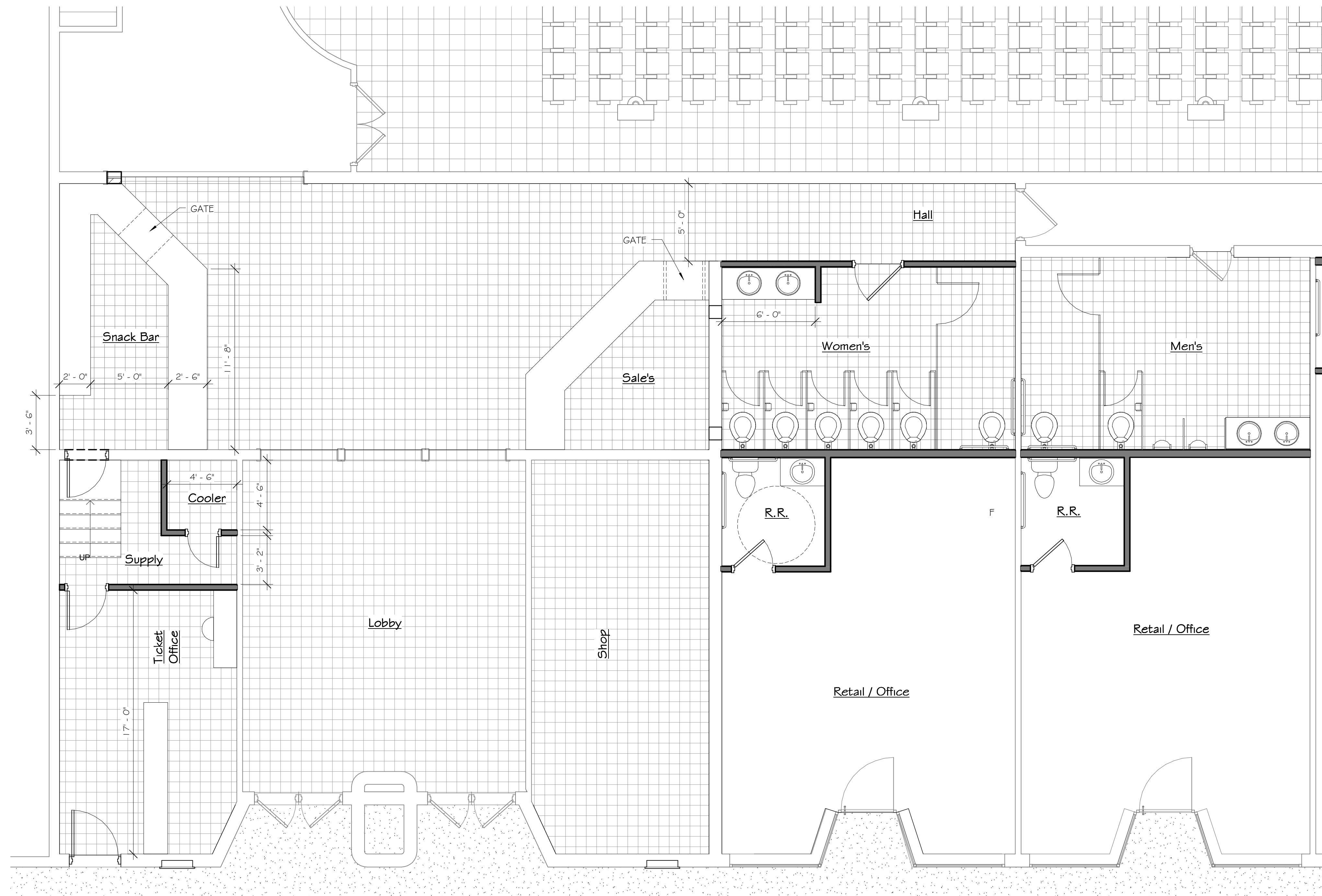
1 Lobby / Lounge Plan - New Work 1/4" = 1'-0"
