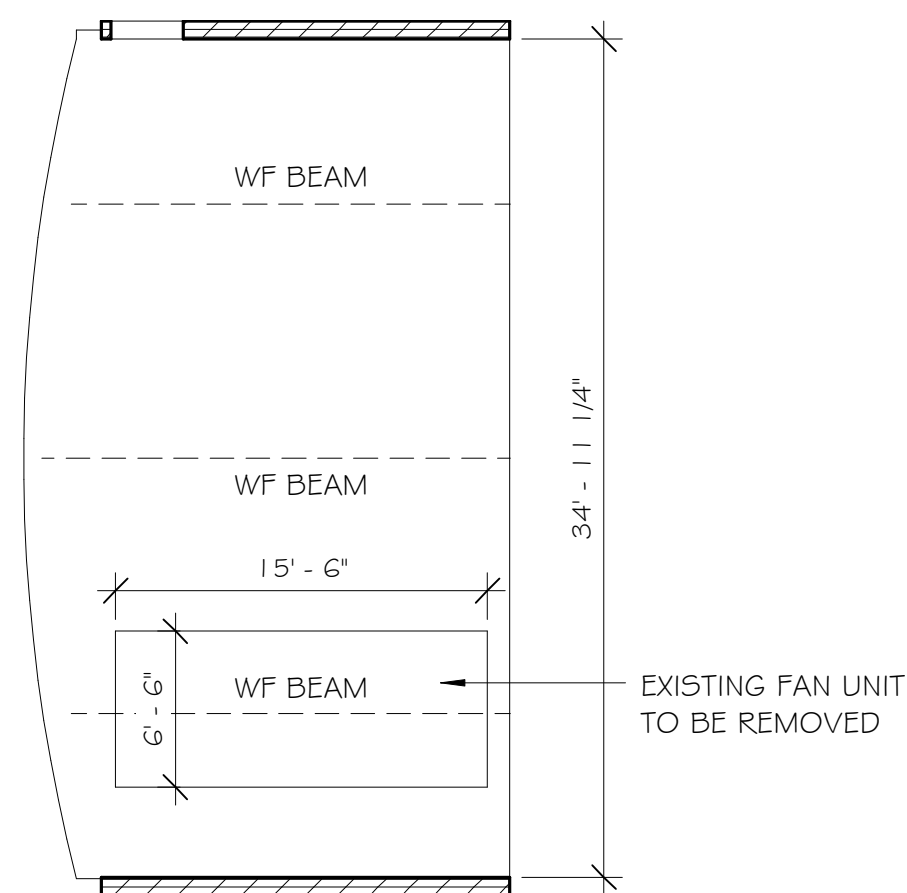
③ Floor Plan Under Stage - Existing / Demolition 1/8" = 1'-0"
