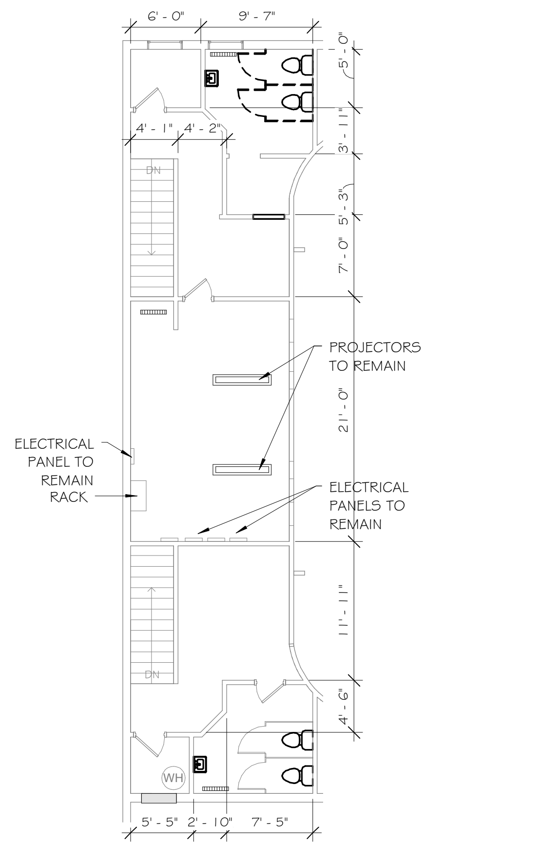
② Projection Level Plan - Existing / Demolition 1/8" = 1'-0"
