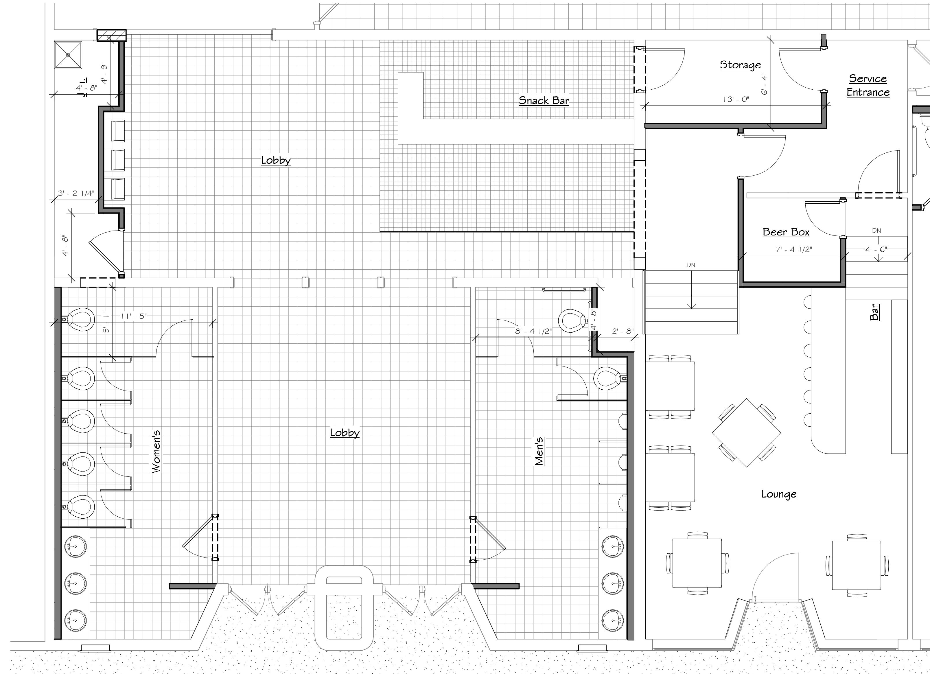
1 Lobby / Lounge Plan - New Work 1/4" = 1'-0"
