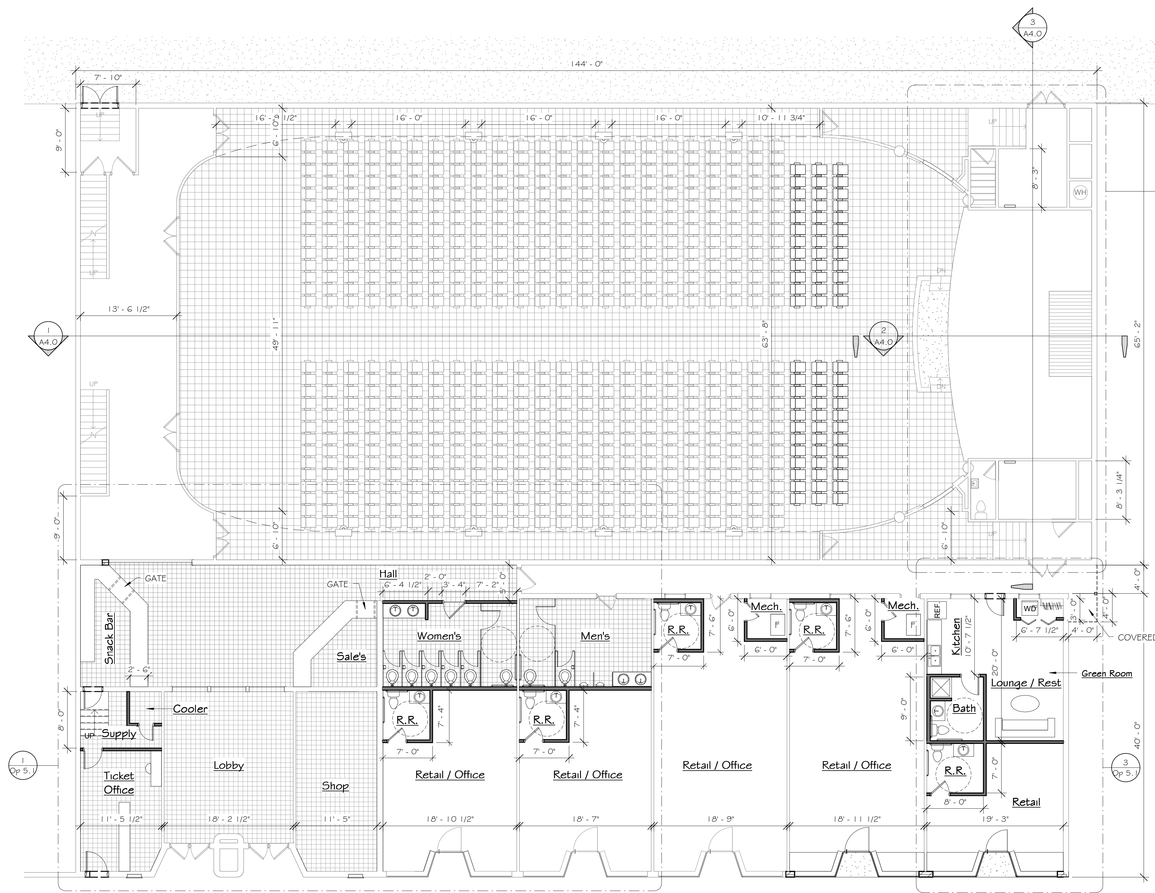
1 First Floor Plan - New Work 1/8" = 1'-0"
