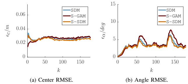
Figure 10: Results for the moving target without occlusion.
