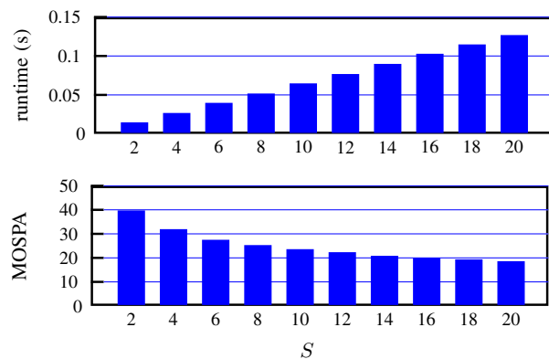
Fig. 6. Runtime per time step (top) and MOSPA (bottom) of the proposed algorithm versus number of sensors for K = 5 intersecting targets.
