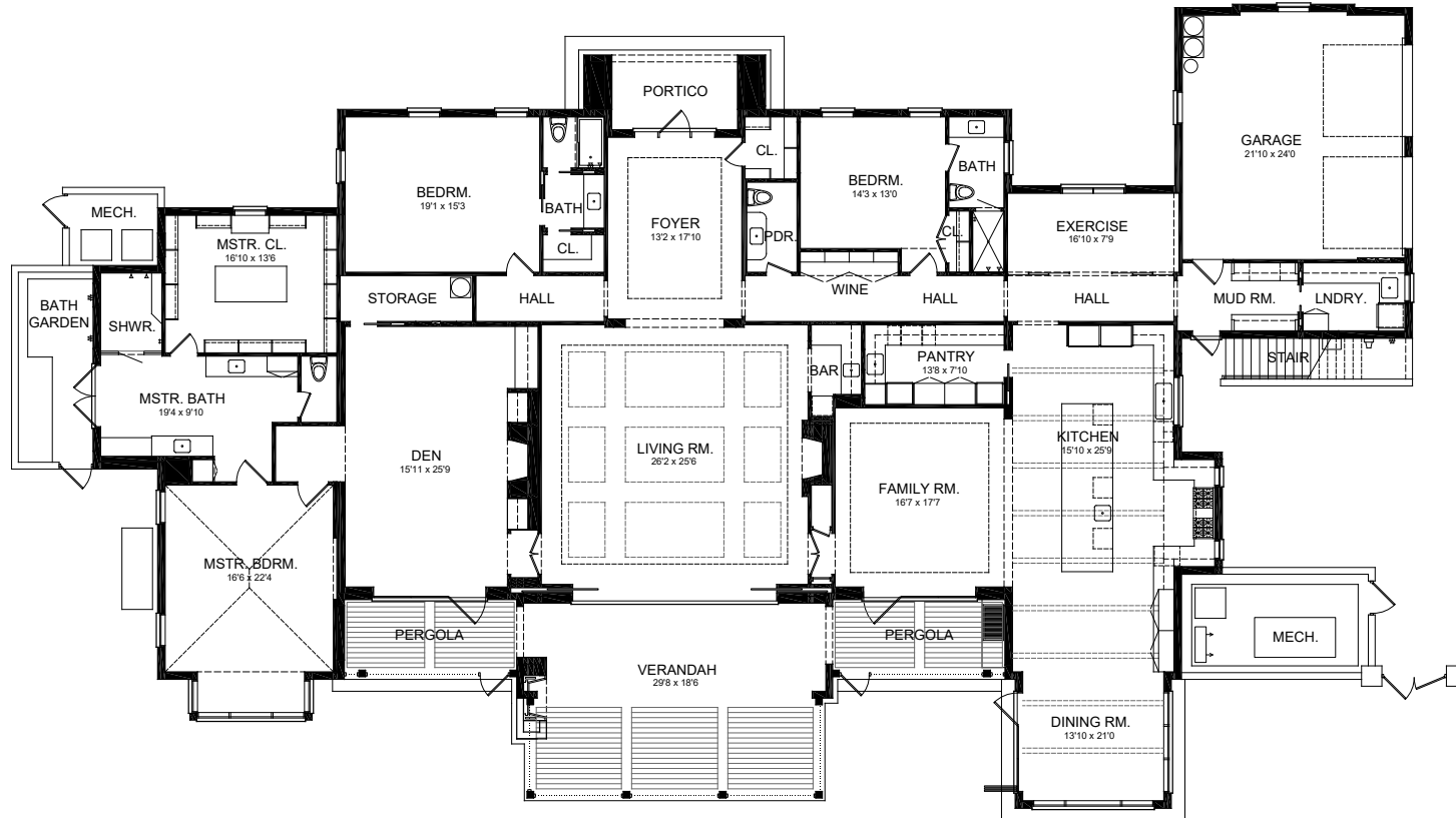
FLOOR PLAN
