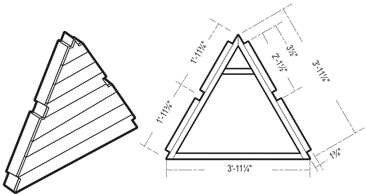
Nest Back Wall (x1) Scale 1:500
