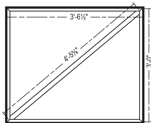
Door measurements
