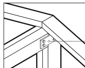
Bolt Plate through rafter and support frame
