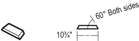
④ General Header (x4) Scale 1:500
