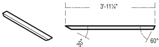
⑤ Side Plate (x8) Scale 1:500
