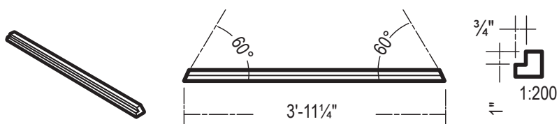
⑦ Bottom Track (x1) Scale 1:500
