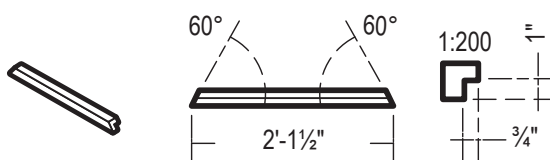
⑨ Top Track (x1) Scale 1:500
