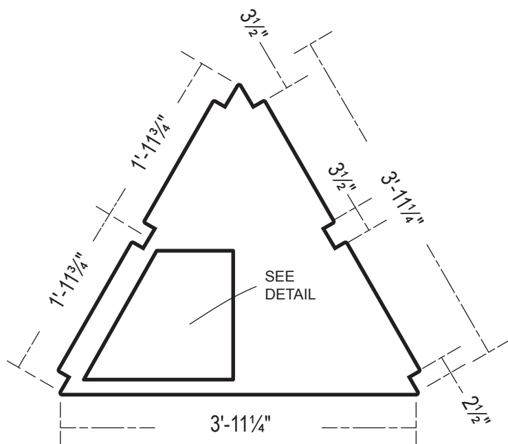
Nest Entrance Sheathing (x2) Scale 1:500
