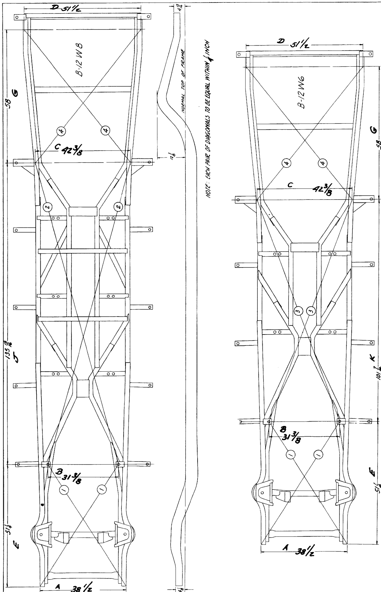
Fig. 2-Frame Straightening Measuring Points Models A-12W6M, A-12W8M
