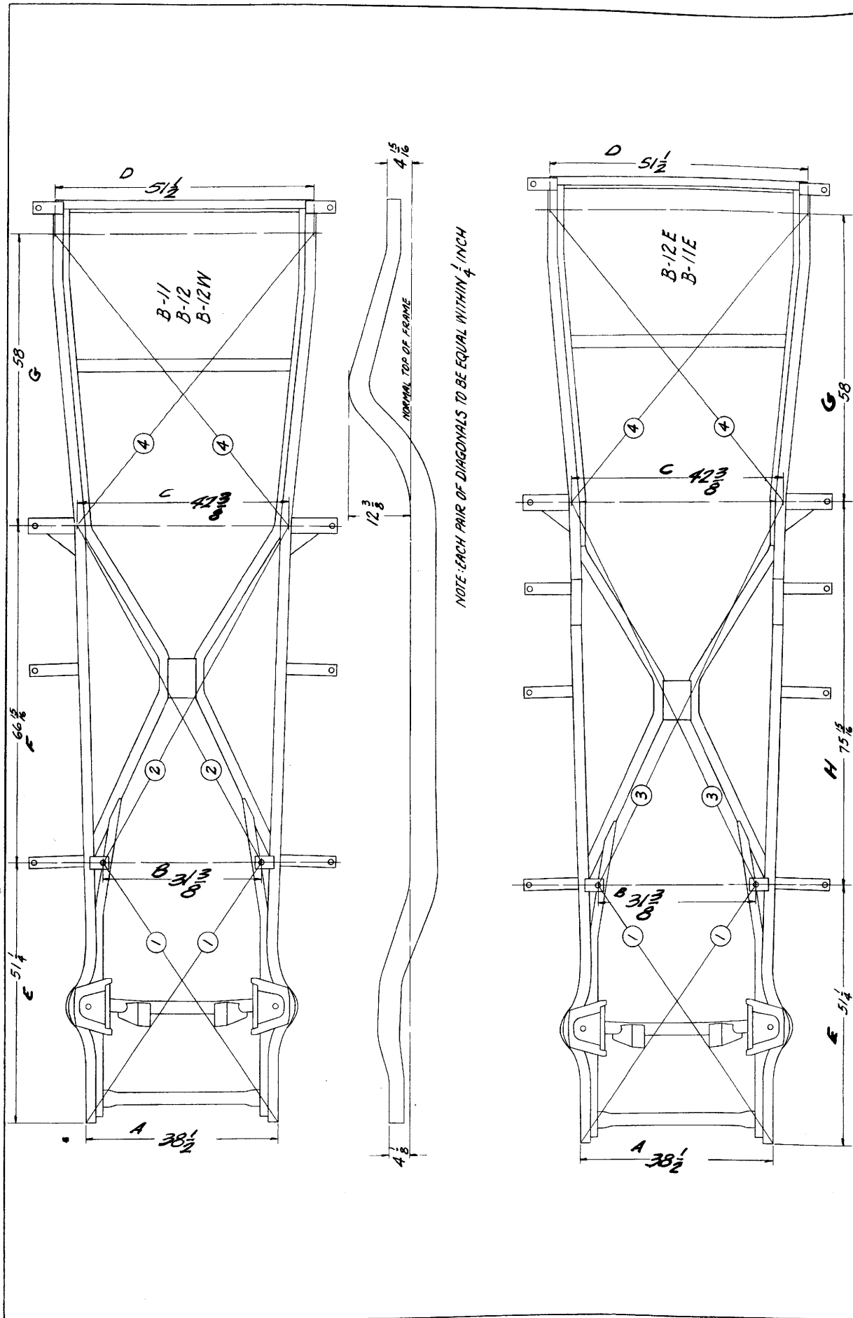
Fig. 1-Frame Straightening Measuring Points Models A-11, A-11E, A-12E, and A-12W After Chassis 20000
