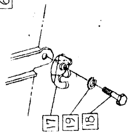
VIEW "C" (TYP. SHIELD ATTACHMENT)
