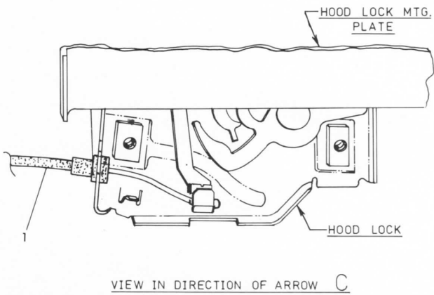
FIGURE 1—Hood Lock Release Installation
