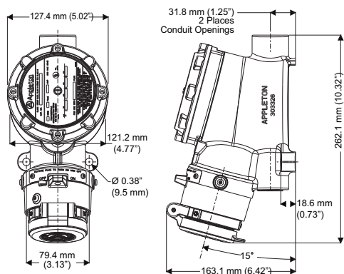
30 Amp
