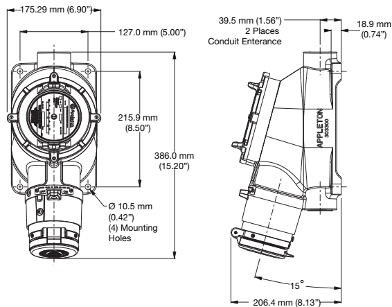
60 Amp
