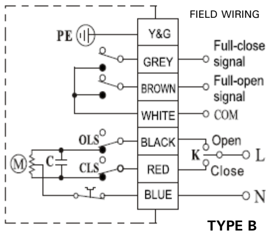
AC Voltage Wiring Diagram
