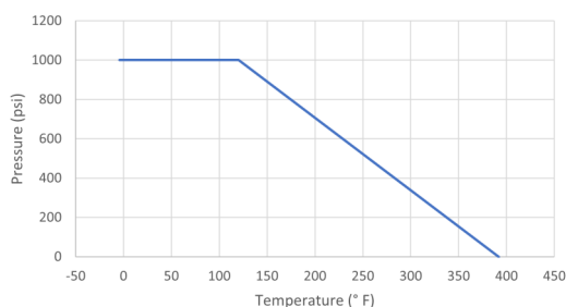
PTFE Pressure vs Temperature- Standard Units
