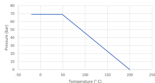
PTFE Pressure vs Temperature- Metric Units
