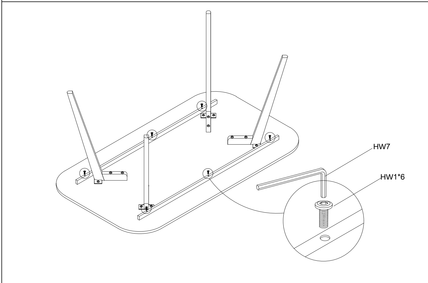
STEP4 assemble table top with metal bar and legs
