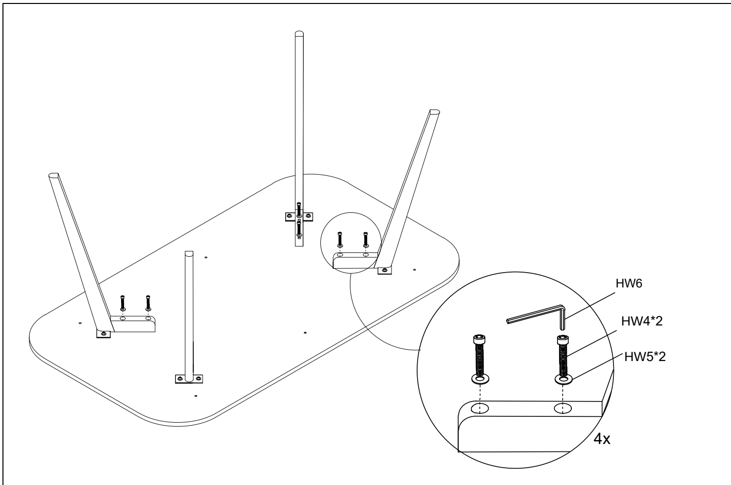
STEP3 assemble legs and metal plate
