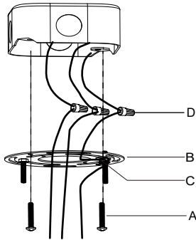
Step 1: Secure mounting plate (B) to outlet box with mounting screws (A).
