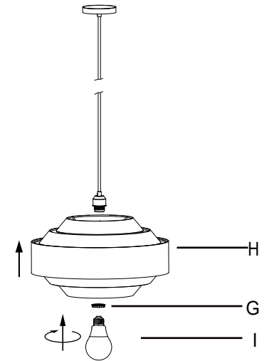
Step 4: Then install shade on the lamp holder and tighten it clockwise with the lamp holder ring (G). Insert the bulb (I) into the bulb holder
