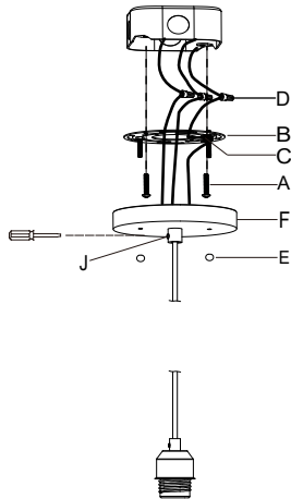
Step 3: Loosen the Allen screw (J) with a screwdriver, adjust it to the required length, attach the canopy of the lamp body (F) onto the mounting plate (B), and secure it with round nut (E).
