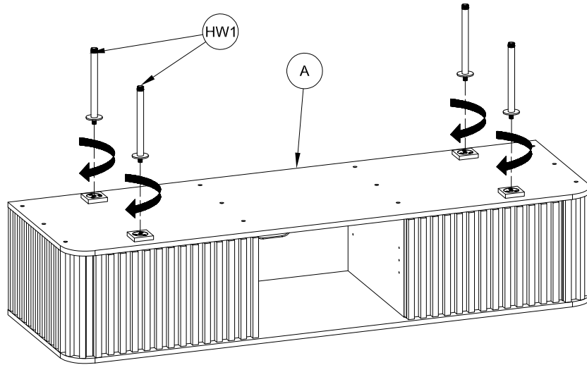
STEP 1: Attach four legs to the cabinet.
