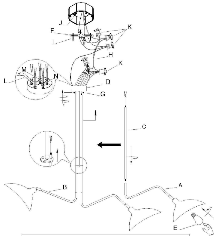
The assembly sequence
