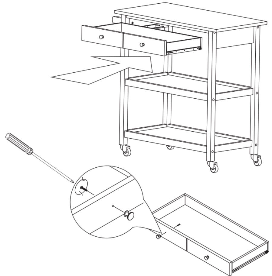
Step 6 : Attach the silver metal knob, then insert the drawer unit through the slider rail.
