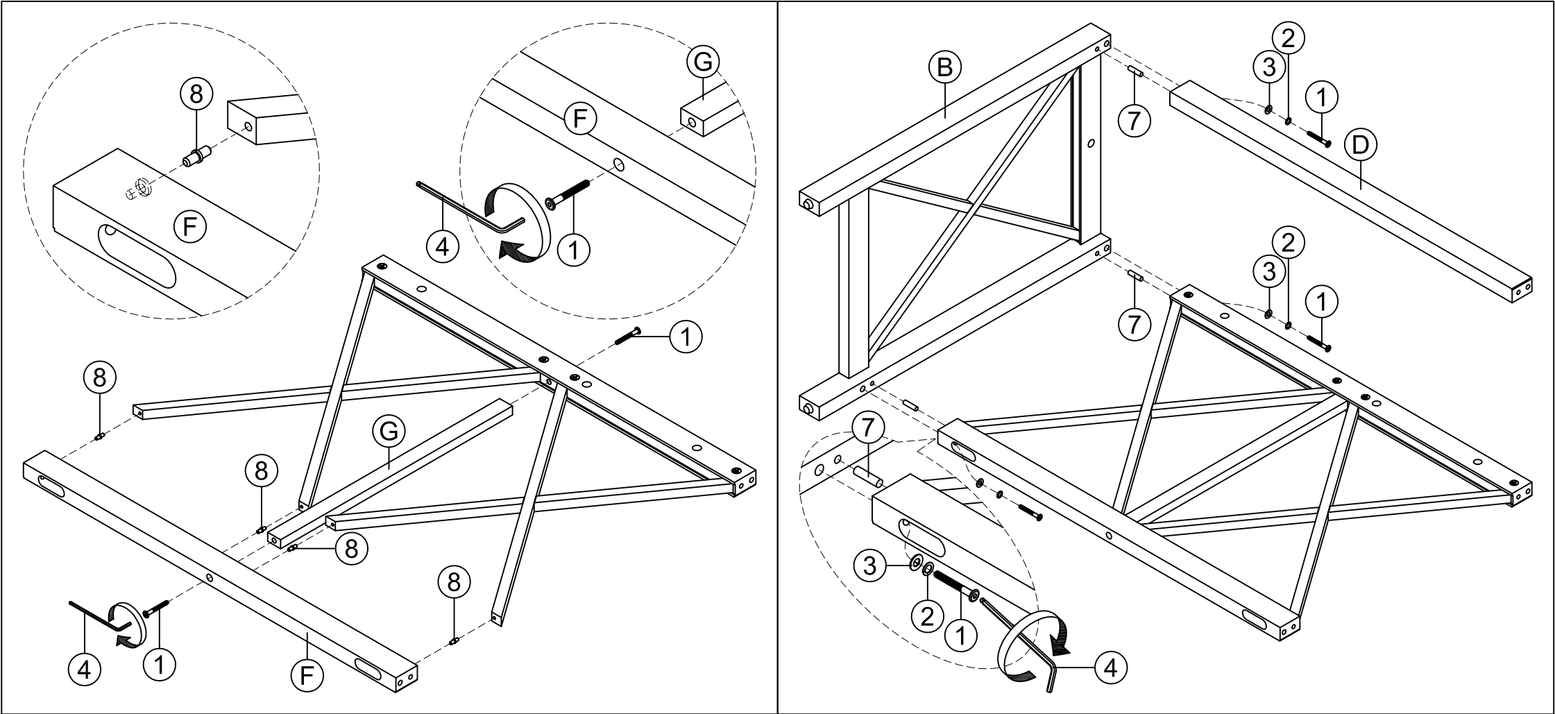
STEP 3 ATTACH VERTICAL RAIL TO UNIT USING 55mm HEAD CAP BOLT. ATTACH BACK BOTTOM RAIL TO UNIT USING 55mm HEAD CAP BOLT AND PINS. TIGHTEN BOLTS USING ALLEN KEY.
