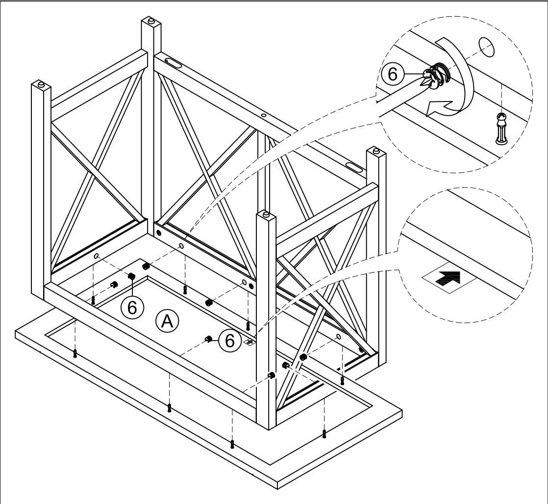
STEP 6 ATTACH TOP PANEL TO UNIT USING CAM LOCKS. NOTE: PAY ATTENTION TO THE POSITION OF THE ARROW LABEL IN THE TOP PANEL.
