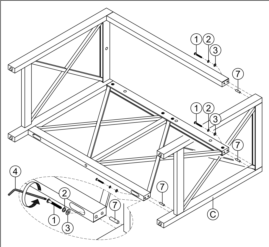
STEP 5 ATTACH UNIT TO RIGHT ASSEMBLY UNIT USING 55mm HEAD CAP BOLTS, SPRING WASHERS AND FLAT WASHERS. TIGHTEN BOLTS USING ALLEN KEY.
