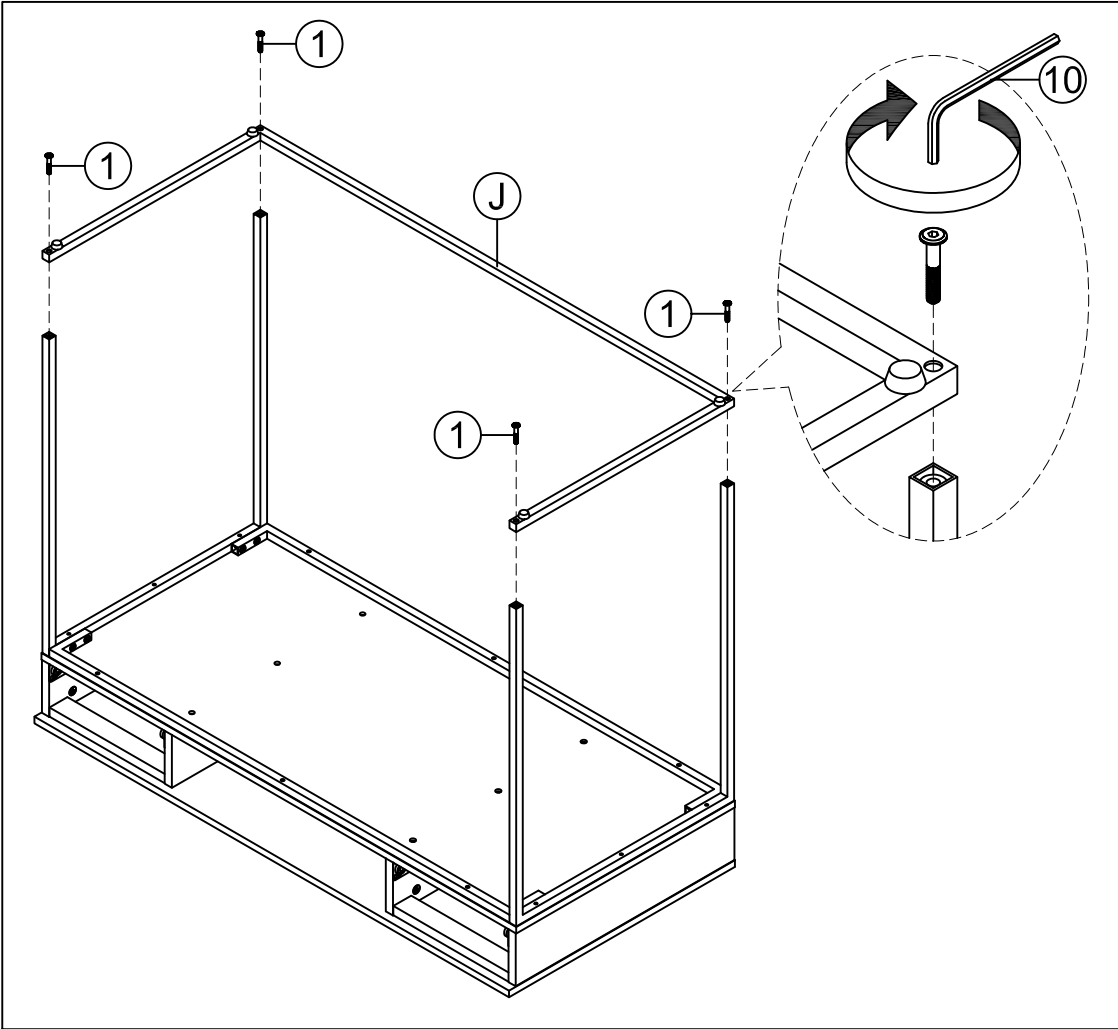
STEP 7 ATTACH BASE FRAME TO UNIT USING 35mm HEAD CAP BOLTS. TIGHTEN BOLTS USING ALLEN KEY.
