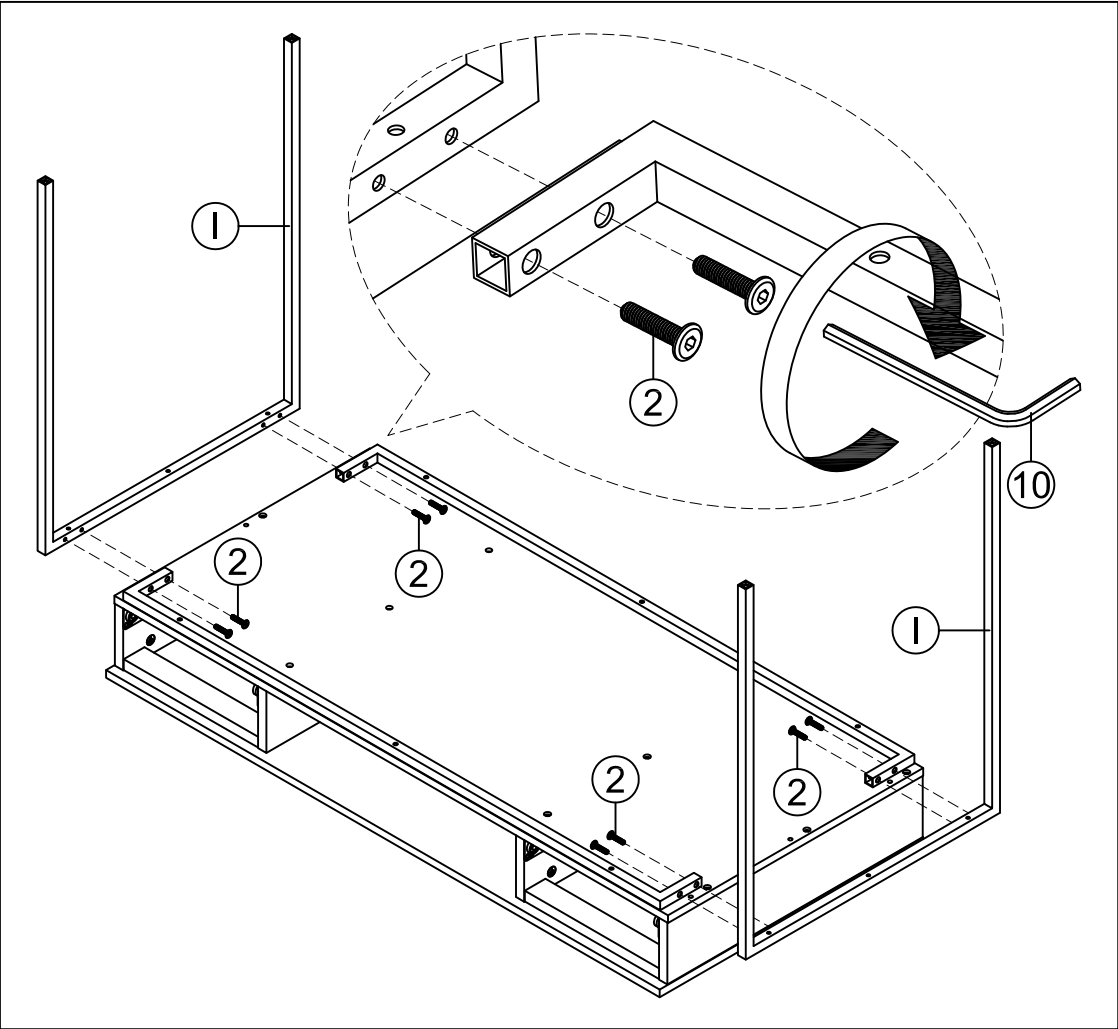
STEP 6 ATTACH LEG FRAMES TO UNIT USING 25mm HEAD CAP BOLTS. NOTE: TURN BOLTS USING ALLEN KEY ONLY HALFWAY THIS TIME.
