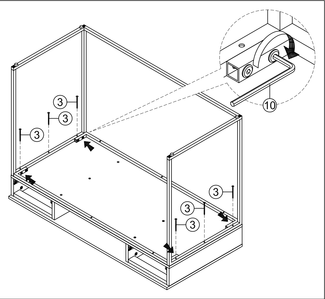
STEP 8 TIGHTEN BOLTS FROM STEP 6 USING ALLEN KEY. ATTACH 1 3/4 ROUND HEAD SCREWS TO UNIT.
