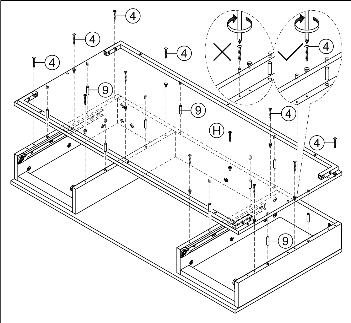
STEP 5 ATTACH BOTTOM PANEL TO UNIT USING 1" ROUND HEAD SCREWS AND DOWELS.
