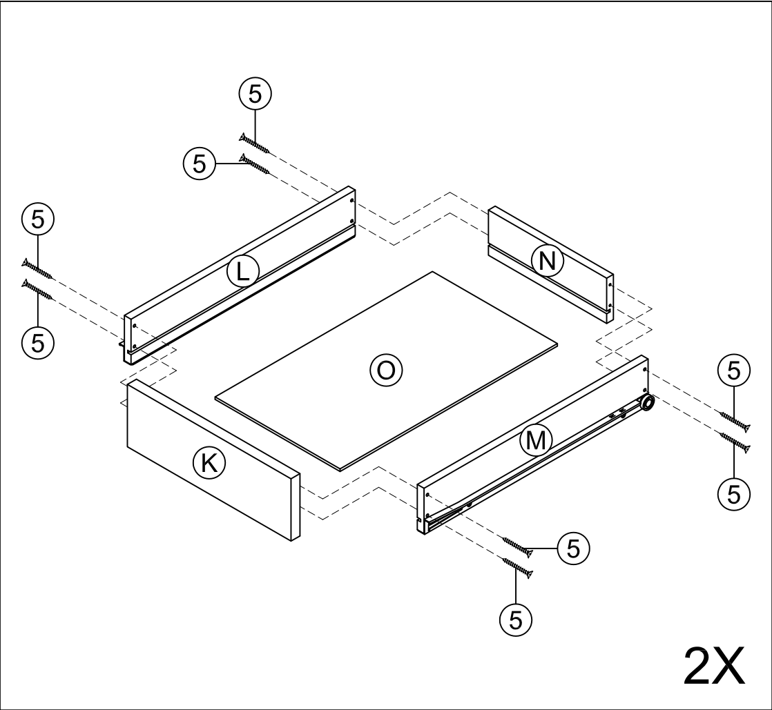
STEP 10 ATTACH DRAWER LEFT AND RIGHT TO DRAWER BACK USING 1 1/4" FLAT HEAD SCREWS. SLIDE DRAWER BASE INTO THE GROOVE. ATTACH DRAWER FRONT TO DRAWER LEFT AND RIGHT USING 1 1/4" FLAT HEAD SCREWS.
