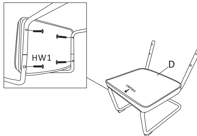
Step 2: SCREW IN THE BOLTS TO ASSEMBLE SEAT PAD(D) AND SEAT FRAME(B). BUT DO NOT TIGHTEN COMPLETELY UNTIL THERE IS NO GAP BETWEEN BACKREST FRAME(A) AND SEAT FRAME(B). ATTENTION TO THE DIRECTION OF FRONT.
