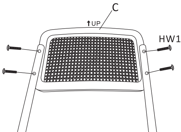
Step 3: SCREW IN THE BOLTS TO ASSEMBLE RATTAN BACKREST(C) AND BACKREST FRAME(A). BUT DO NOT TIGHTEN COMPLETELY. ATTENTION TO THE DIRECTION OF UP AND DOWN
