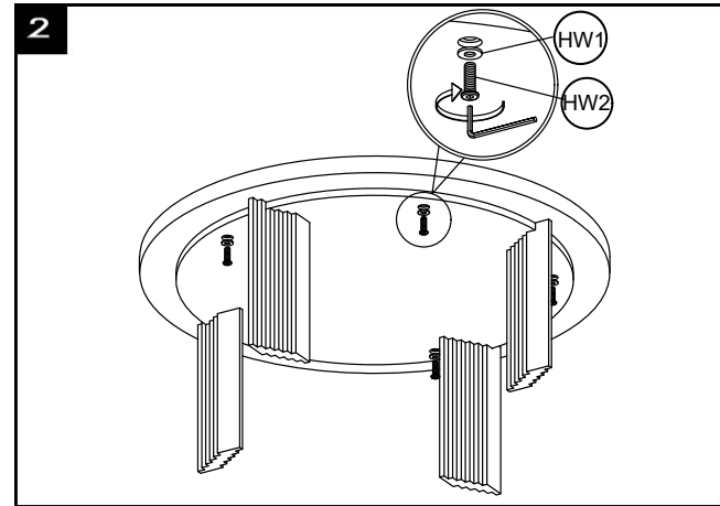
Step 2 : Use bolts M8x30 (HW2) and washer (HW1) to connect the MDF + Paper top
