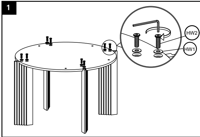
Step 1 : Use bolts M8x30 (HW2) and washer (HW1) to connect the MDF + legs
