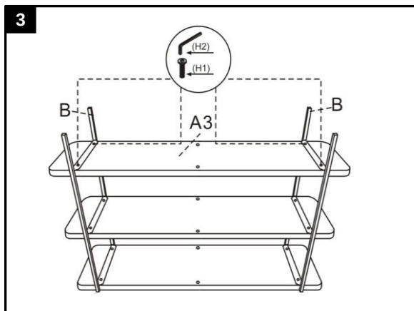
Step 1 Attach the Shelf(A3) to the Metal frame(B), using Allen bolt (H1) Tighten with Allen key(H2)
