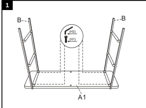
Step 1 Attach the Shelf(A1) to the Metal frame(B), using Allen bolt (H1) Tighten with Allen key(H2)
