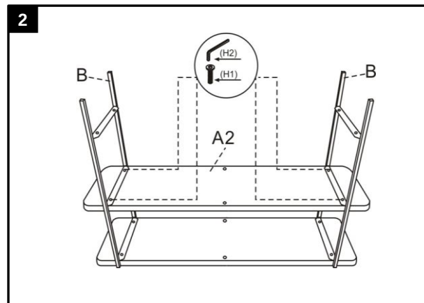
Step 2 Attach the Shelf(A2) to the Metal frame(B), using Allen bolt (H1) Tighten with Allen key(H2)
