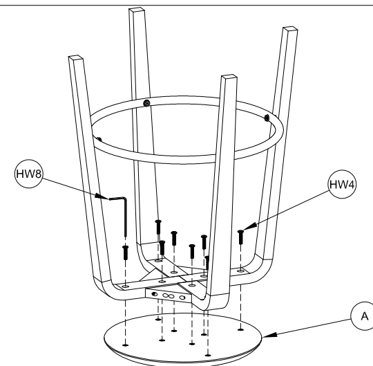
STEP 4: Attach the legs to the seat. Make sure to apply all the bolts into the holes properly before tightening.
