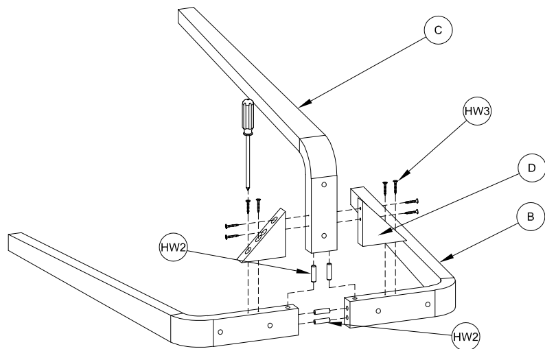
STEP 1: Attach the corner block to the legs.
