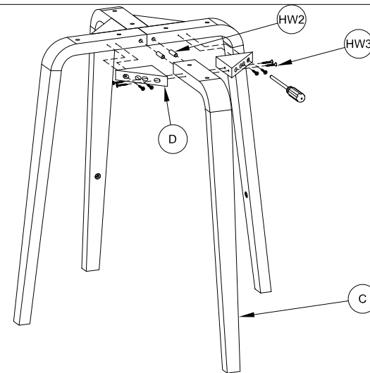
STEP 2: Attach the corner block to the legs.
