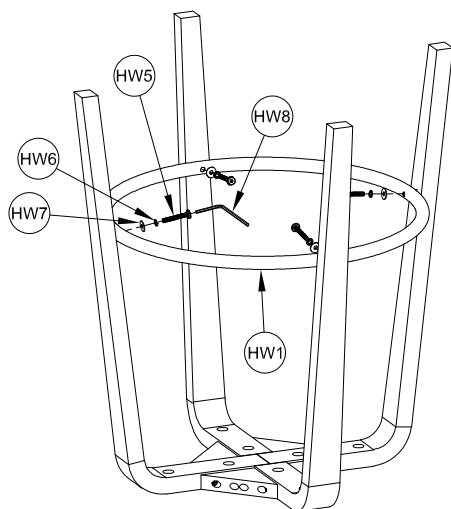
STEP 3: Attach the iron brackets to the legs.
