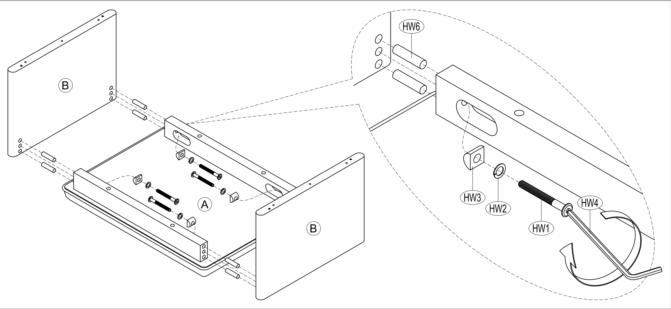
STEP 1 ATTACH CUSHION (A) TO SIDE PANELS (B) USING 55 MM BOLTS (HW1), SPRING WASHERS (HW2), SPACERS (HW3) AND DOWELS (HW6). TIGHTEN BOLTS USING ALLEN KEY (HW4).
