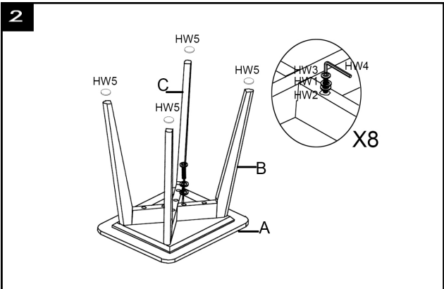
Step2:Attach the cross legs to top plate(A), using 8 split lock washer(HW1) and 8 flat washer(HW2) and 8 socket bolts(HW3). Screw on all bolts and tighten in the end by using allen key(HW4). Put on the felt pad(HW5).
