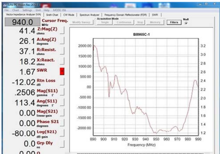
Echo Test antenna #1 with Cable Null ON to eliminate the test lead
