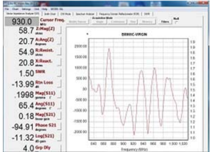
Echo Test antenna #1 with Cable Null OFF
