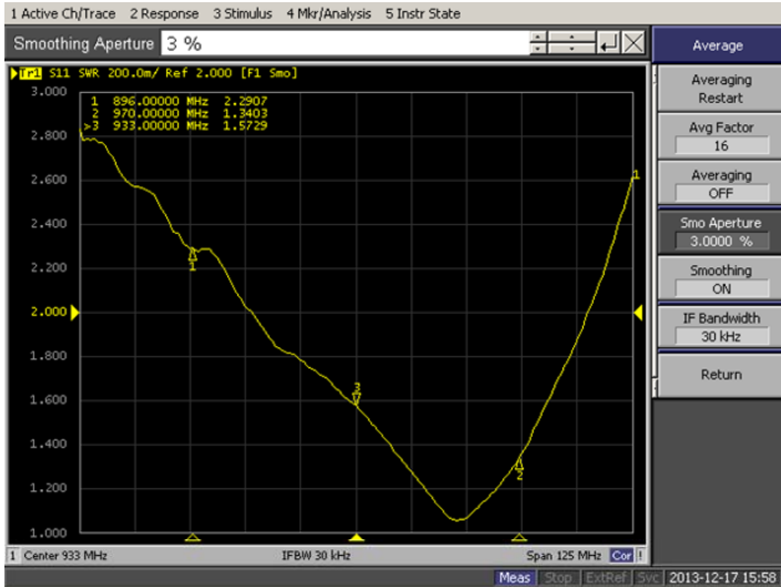
Factory Test on typical production antenna with smoothing on
