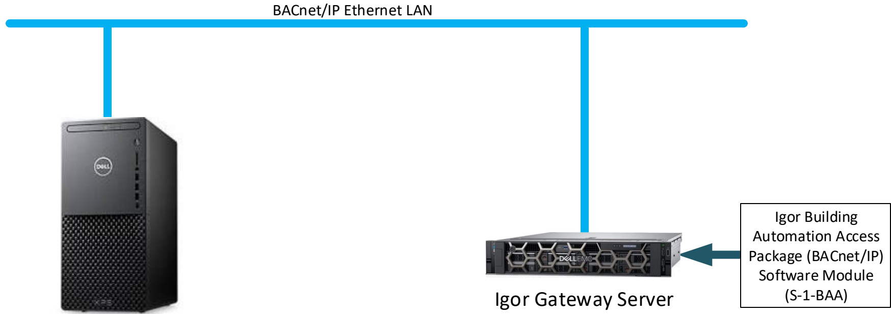
HVAC Control Server (with BACnet/IP Communication)
