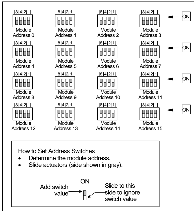
Figure 3: 5414 Digital Input Module Address Switches
