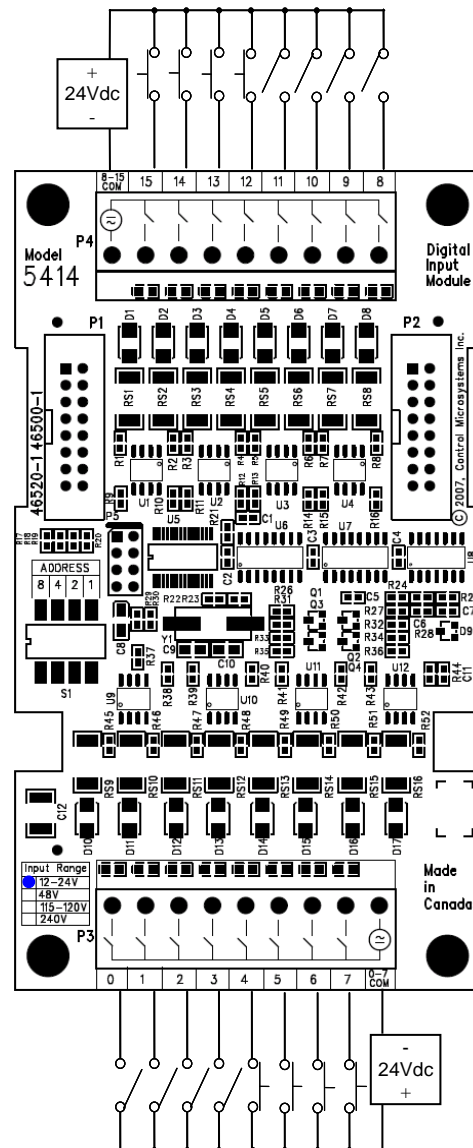
Figure 2: DC Input Wiring Example
