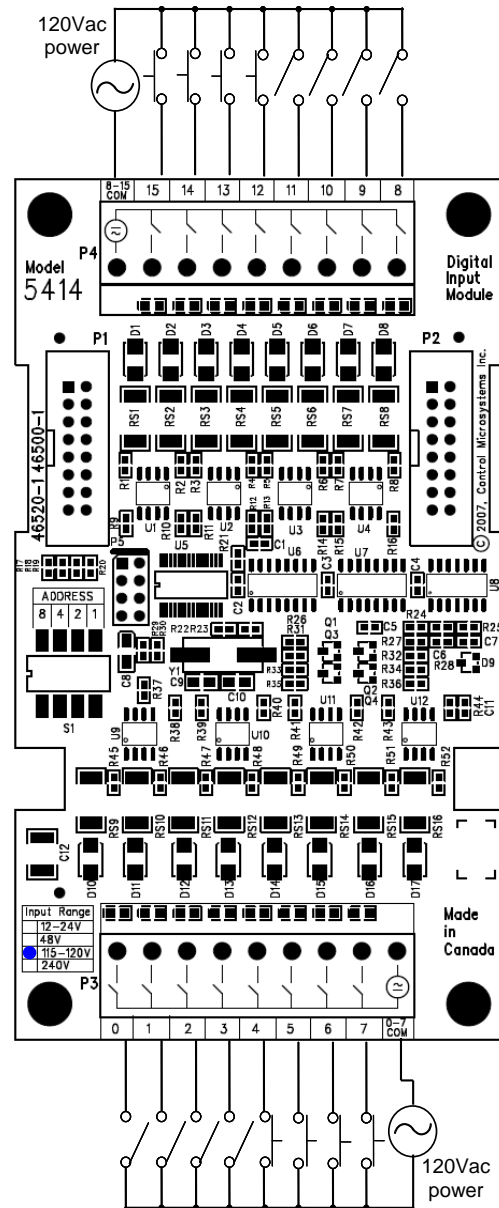
Figure 1: AC Input Wiring Example
