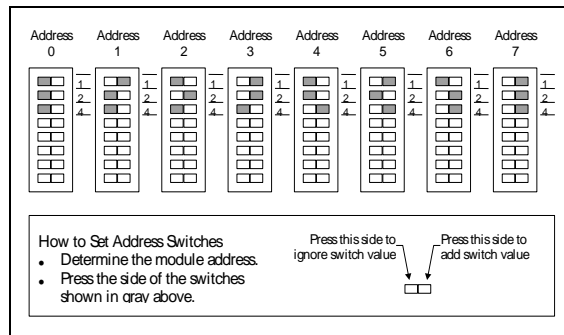
Figure 1: Digital I/O Module Address Switches
