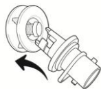
Figure 3 Insert locking pump connector
