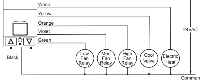
Wiring Diagram 2-pipe Fan Coil with Electric Heat
