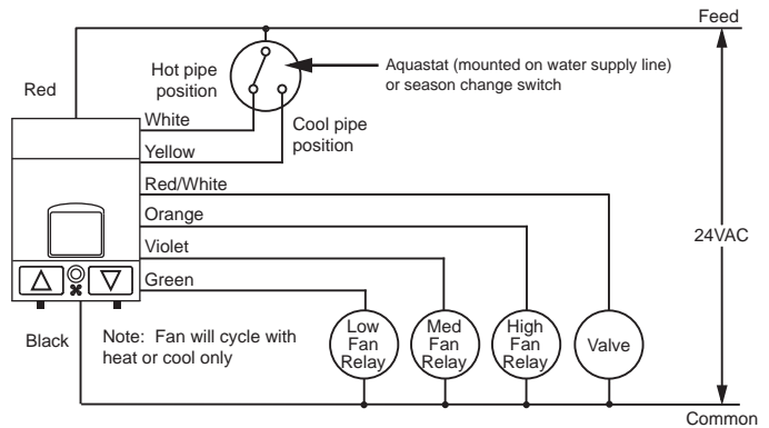
Wiring Diagram 2-pipe Fan Coil with Aquastat
