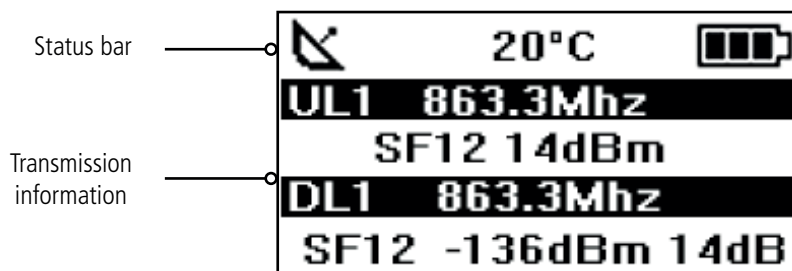
Figure 8 : Principal screen
