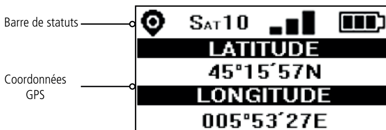
Figure 9 : Ecran GPS
