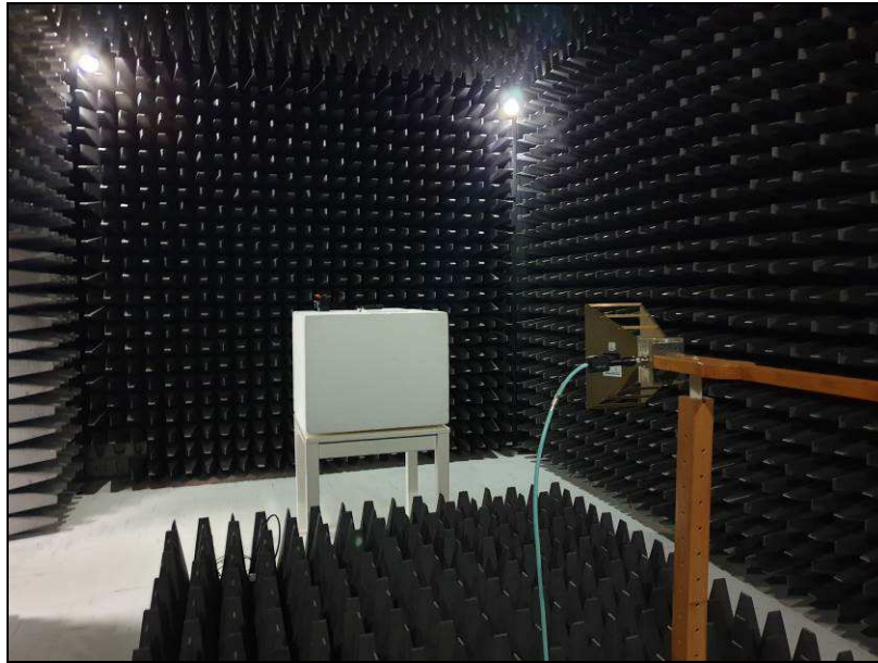
EN 55032 / CISPR 32: Radiated emissions test set-up
