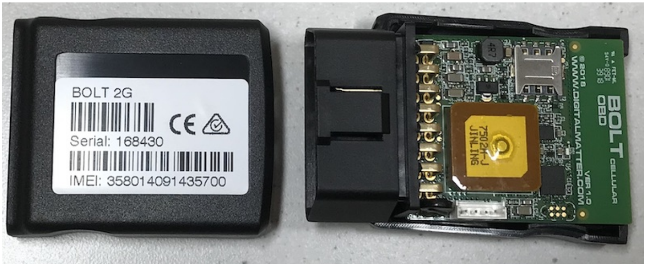
Bottom View: Bolt 2G PCB
