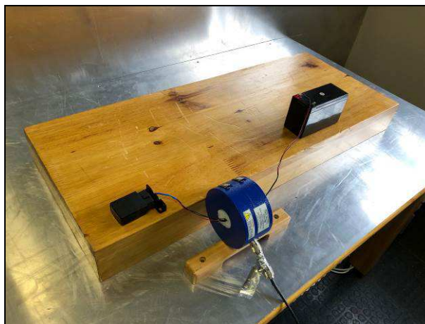
EN / IEC 61000-4-6: Conducted immunity test set-up
