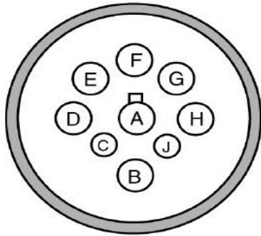
9 Pin Connector
