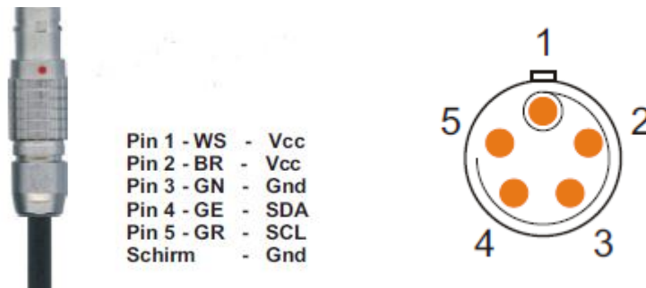
Figure 1 LEMO male connector pinning
