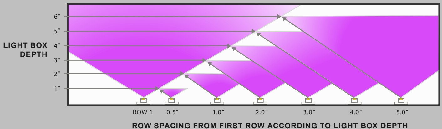
120° LED BEAM ANGLE DIFFUSION DISTANCE
