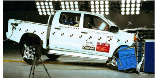
Frontal offset test at 64 km/h (dual cab tested)
