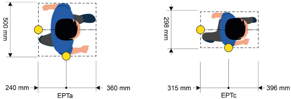
Figure 1.2.1: Virtual box dimensions around EPTa and EPTc
