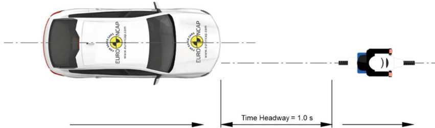
Figure 3-4 CMRb scenario, representing the 25% impact location
