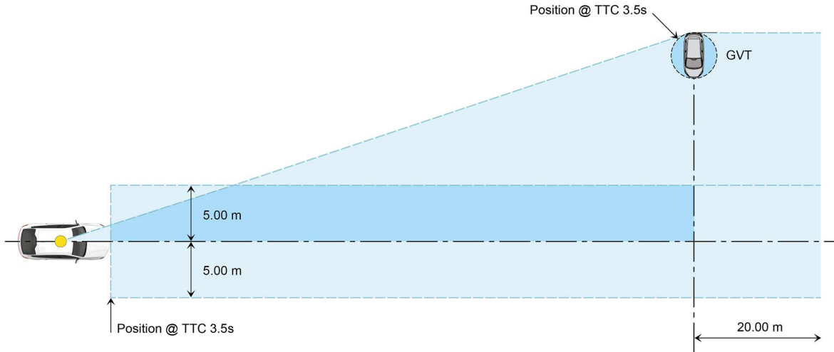
Figure 2-1 Free space requirements – CCCscp Farside Test
