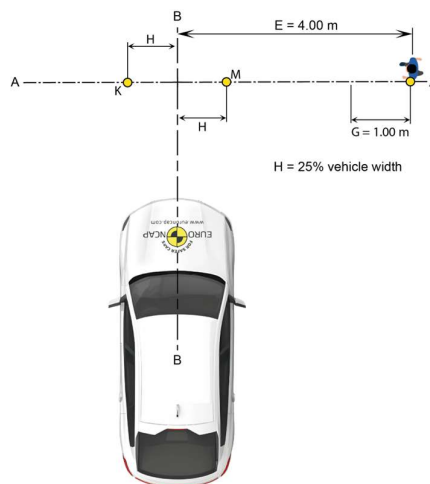
Figure 3-20 CPNA-25 & CPNA-75 scenarios, Walking Adult from Nearside
