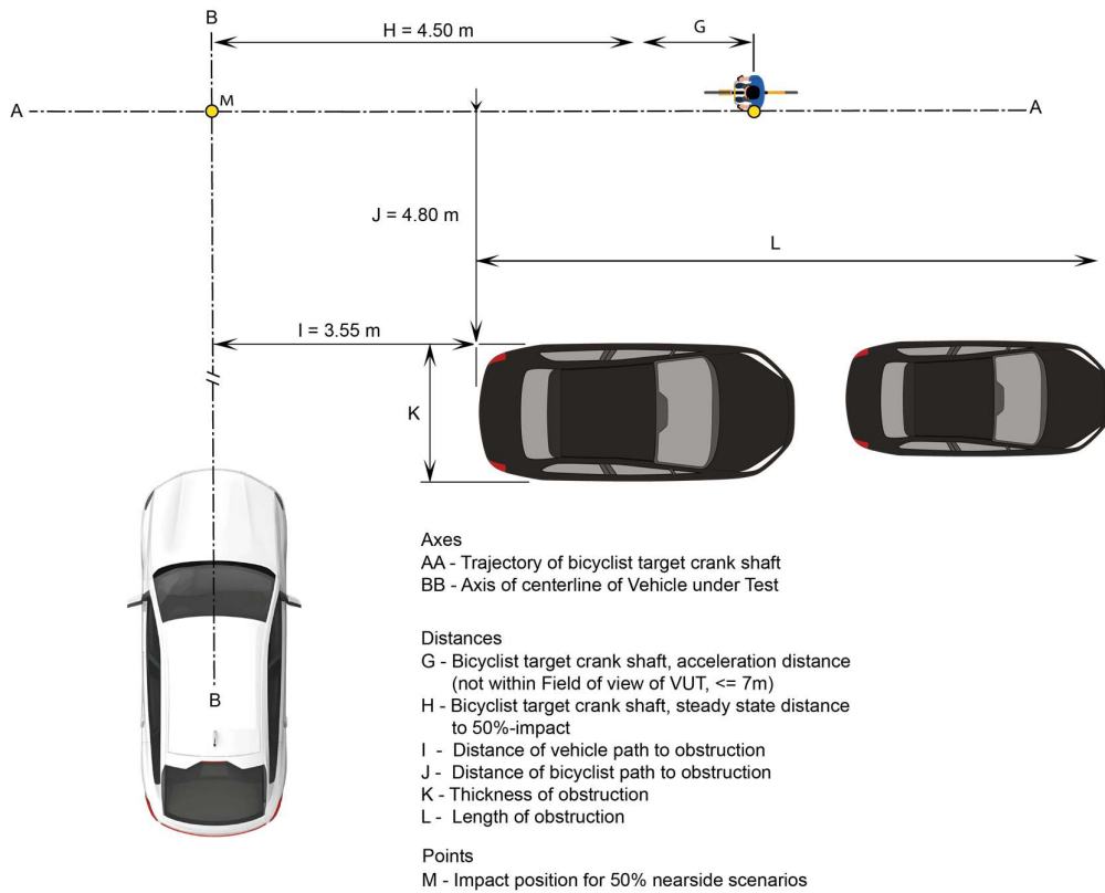
Figure 3-24 CBNAO scenario, Bicyclist from Nearside (obstructed)
