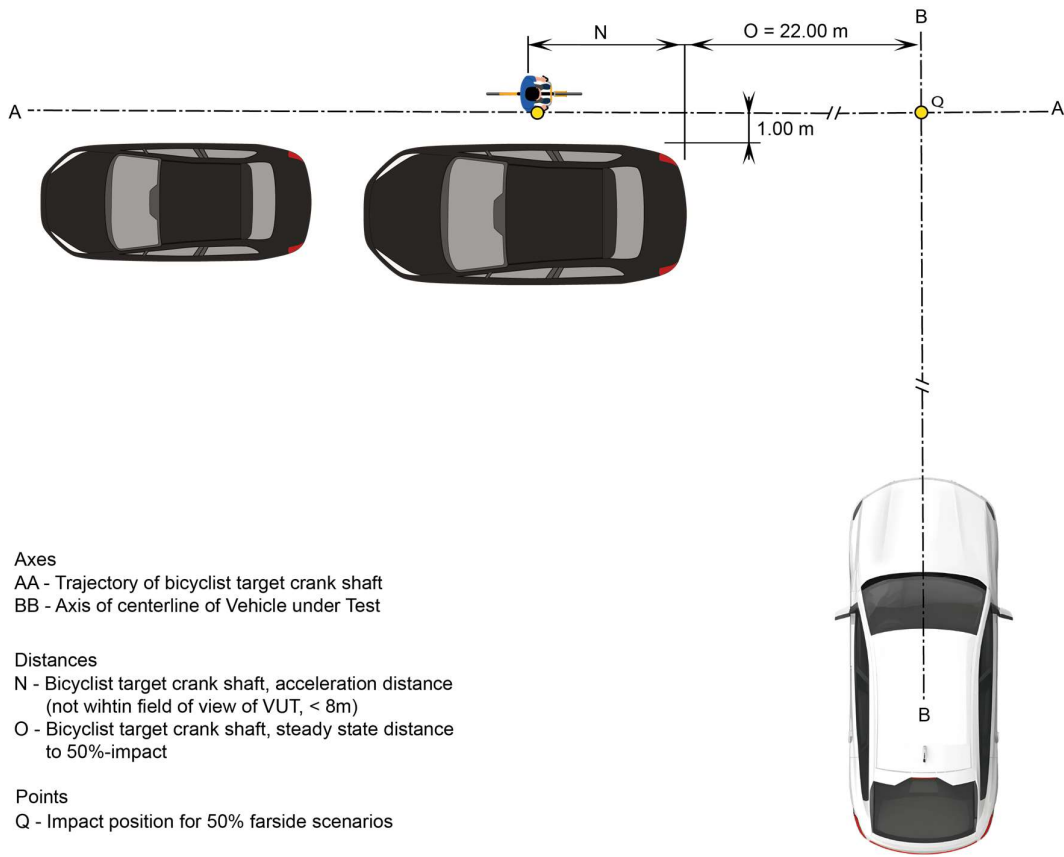
Figure 3-25 CBFA scenario, Bicyclist from Farside
