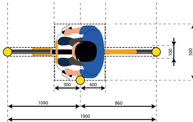
Figure 1.2.2: Virtual box dimensions around EBT
