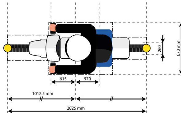
Figure 1.2.3: Virtual box dimensions around EMT
