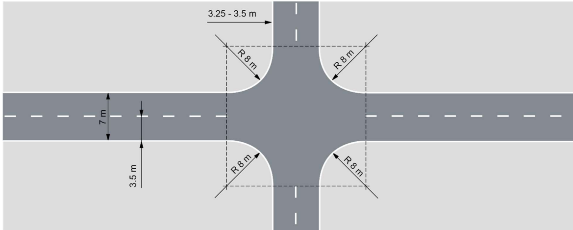
Figure 4.2: Layout of junction and the connecting lanes
