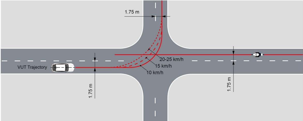
Figure 3-7 CMFtap scenario VUT and EMT paths
