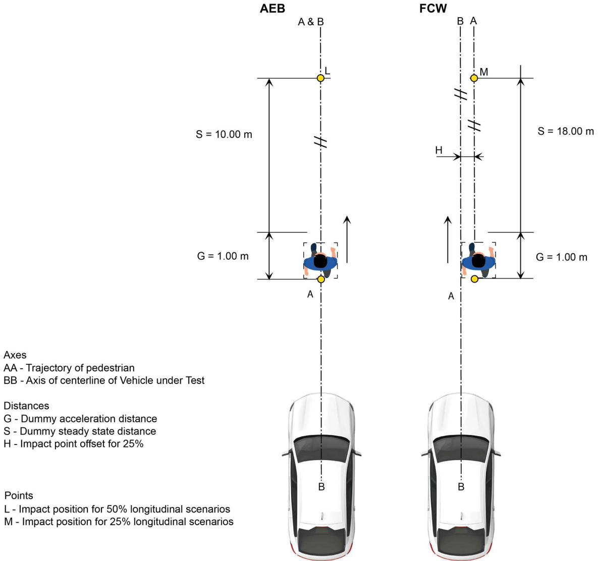
Figure 3-13 CPLA scenario, Longitudinal walking Adult
