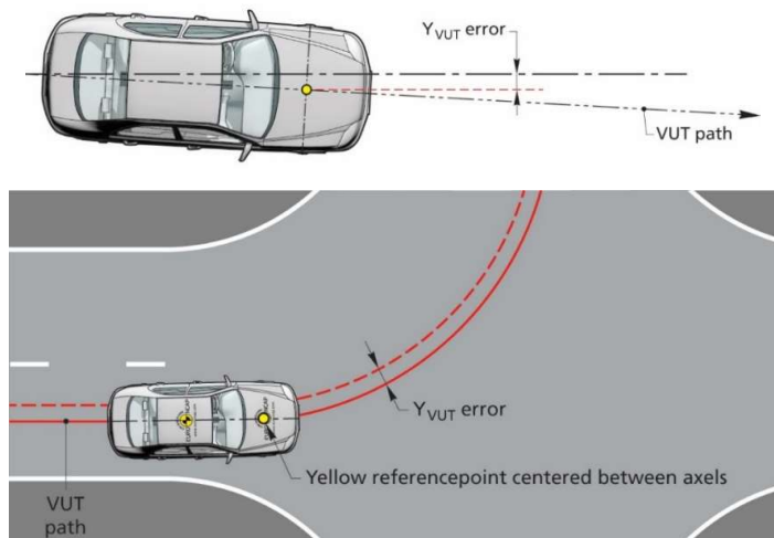
Figure 1-2 VUT Lateral Path Error
