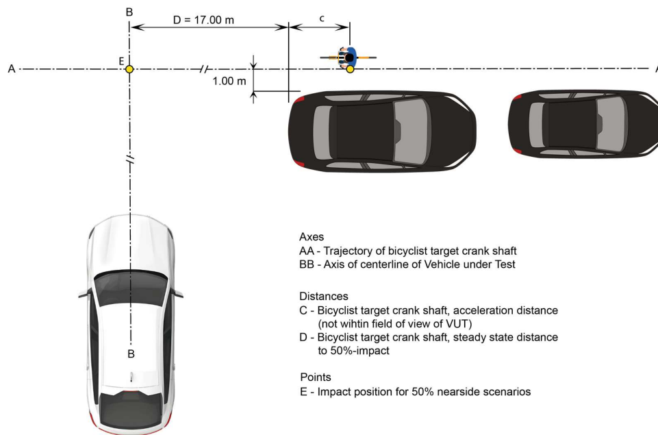
Figure 3-23 CBNA scenario, Bicyclist from Nearside
