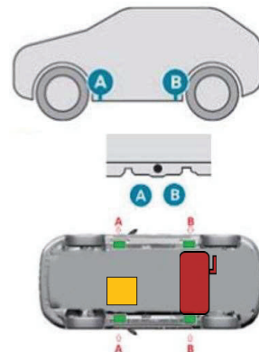
Stabilization/lifting points
