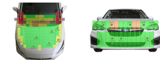
Adult leg impact (upper and full legforms)
