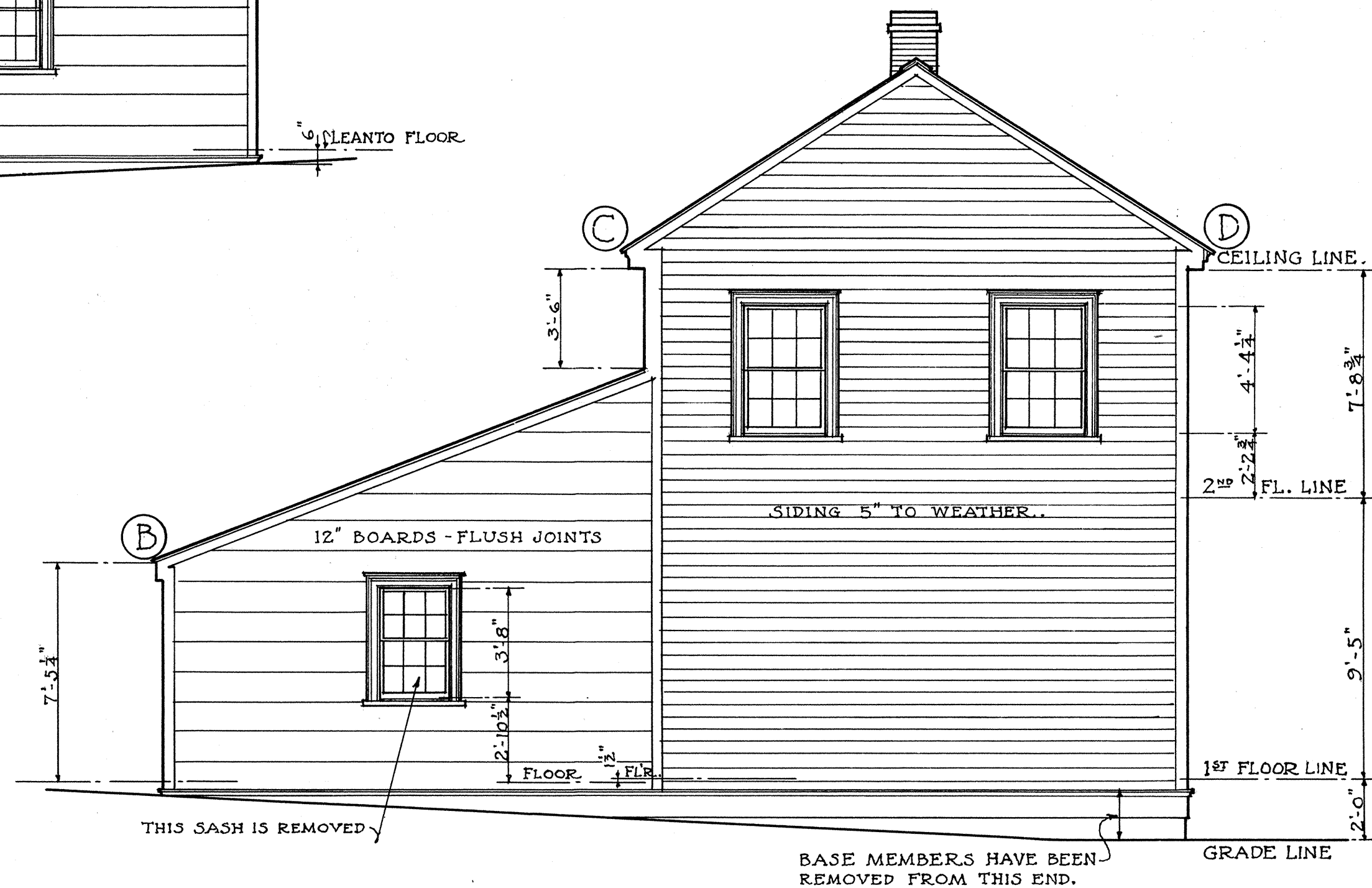
· SOUTH · ELEVATION · SCALE 1/4 INCH = 1 FT.
