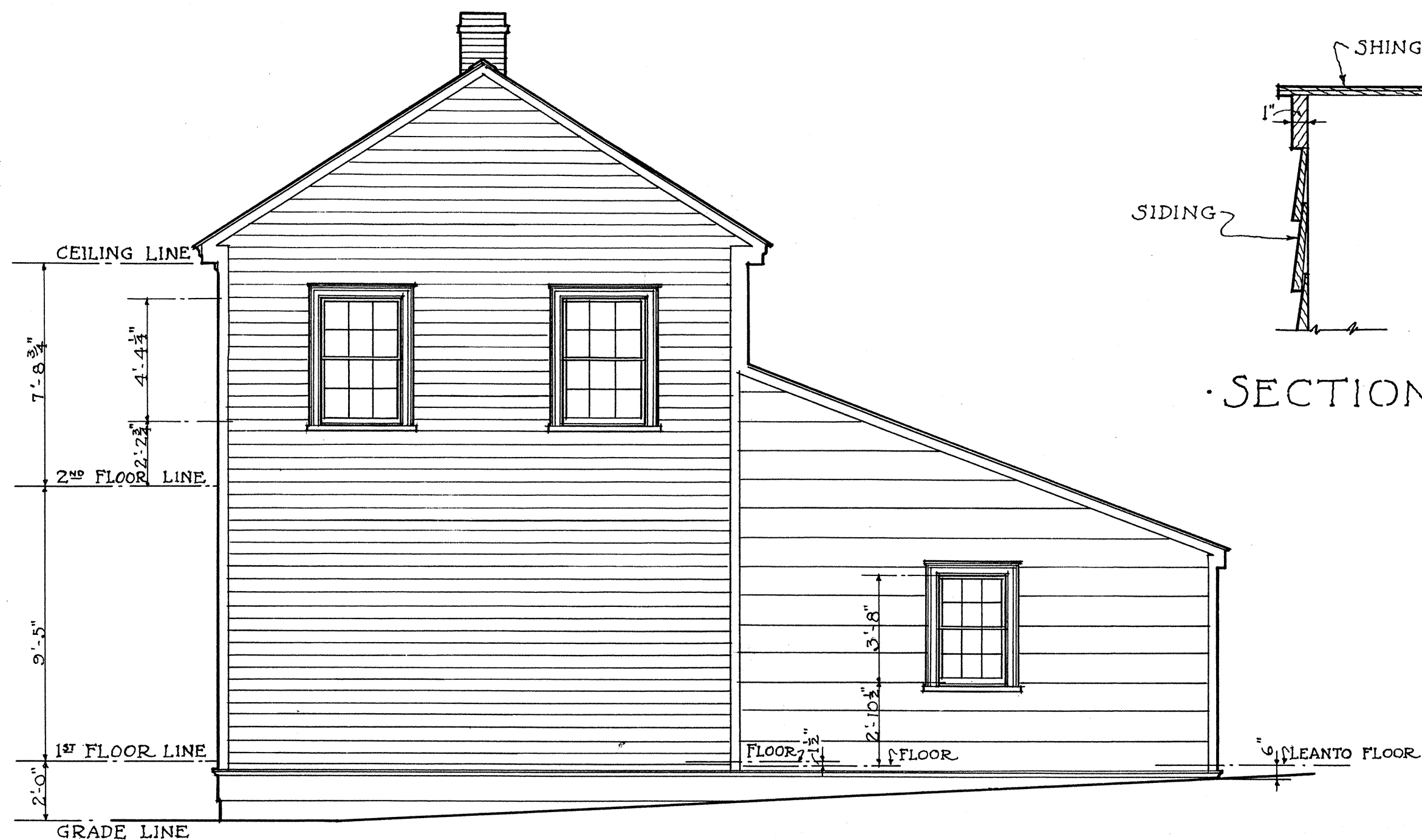
· NORTH · ELEVATION · SCALE 1/4 INCH = 1 FT.
