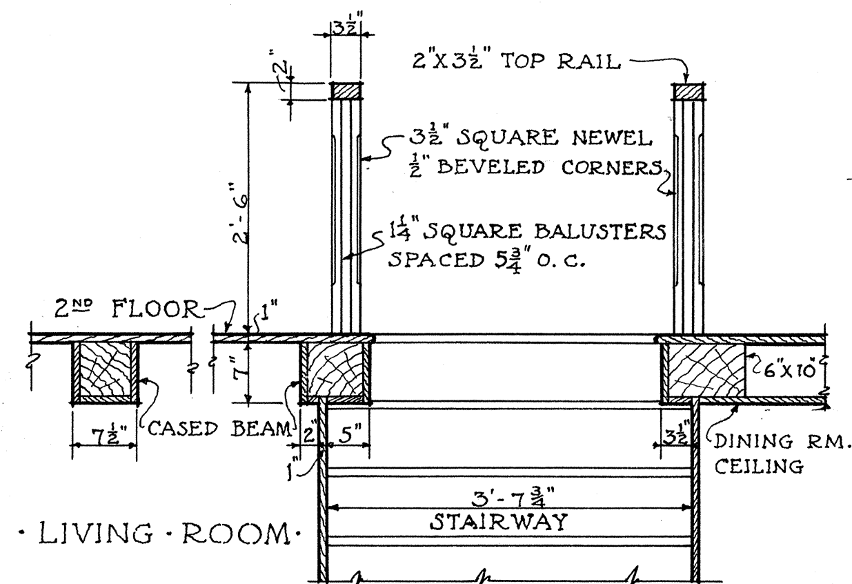
SECTION THRU 2 ND FLOOR AND STAIRWAY AT F-F
