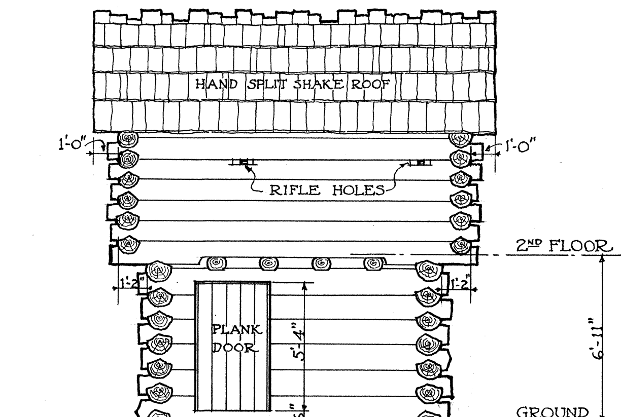
• NORTHWEST • ELEVATION •
