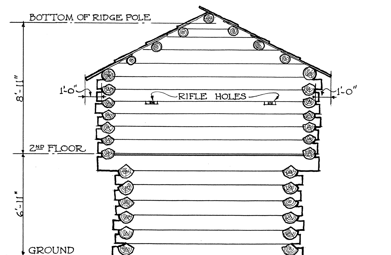
• SOUTHWEST • ELEVATION •
