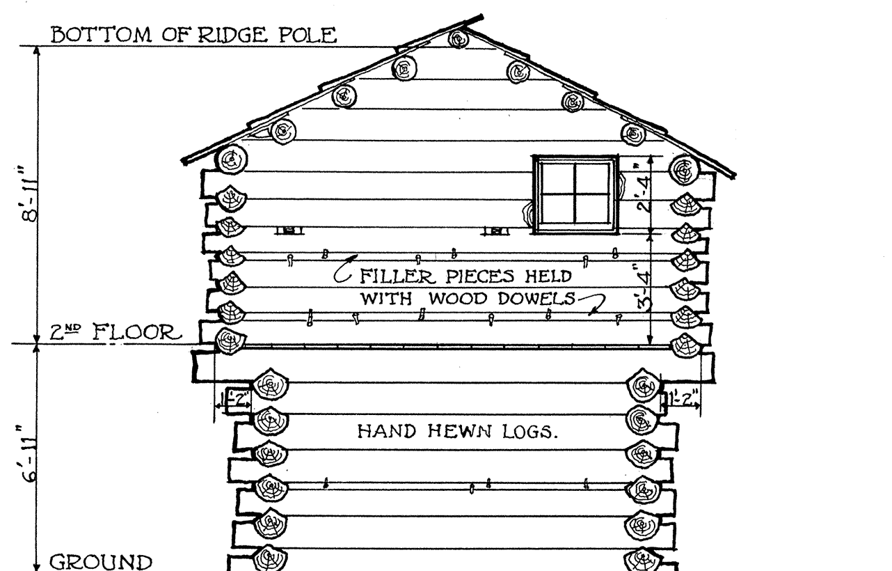
• NORTHEAST • ELEVATION •
