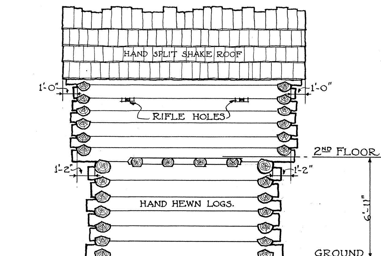
• SOUTHEAST • ELEVATION •
