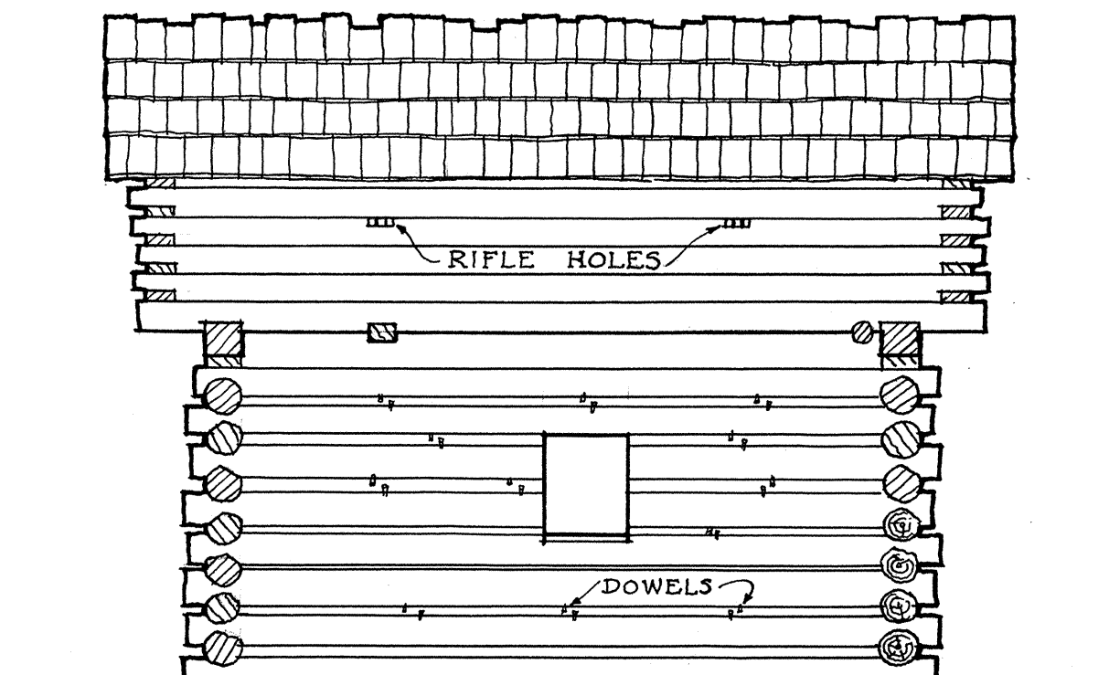
· NORTHWEST · ELEVATION ·
