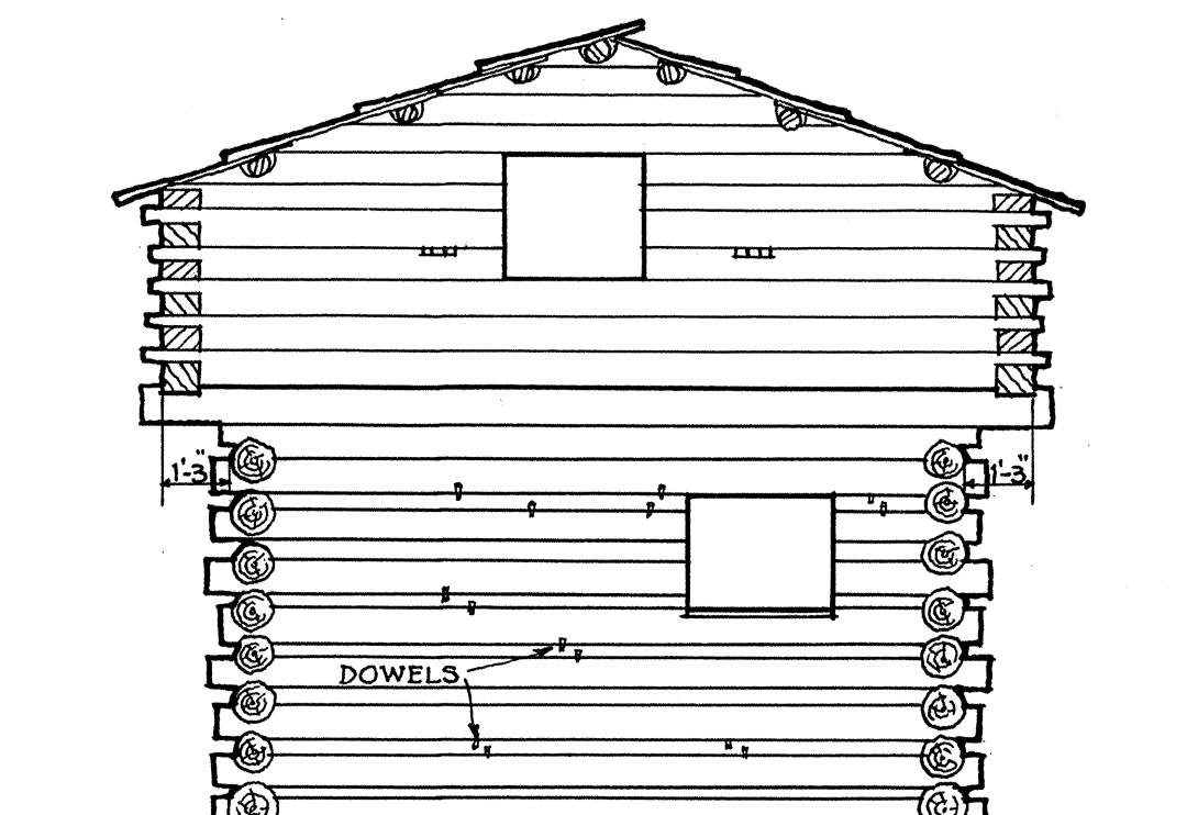
· SOUTHWEST · ELEVATION ·
