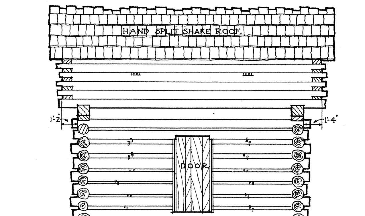
· SOUTHEAST · ELEVATION ·
