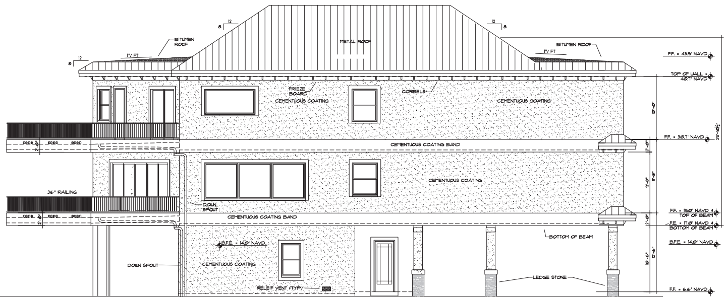
Left Elevation
