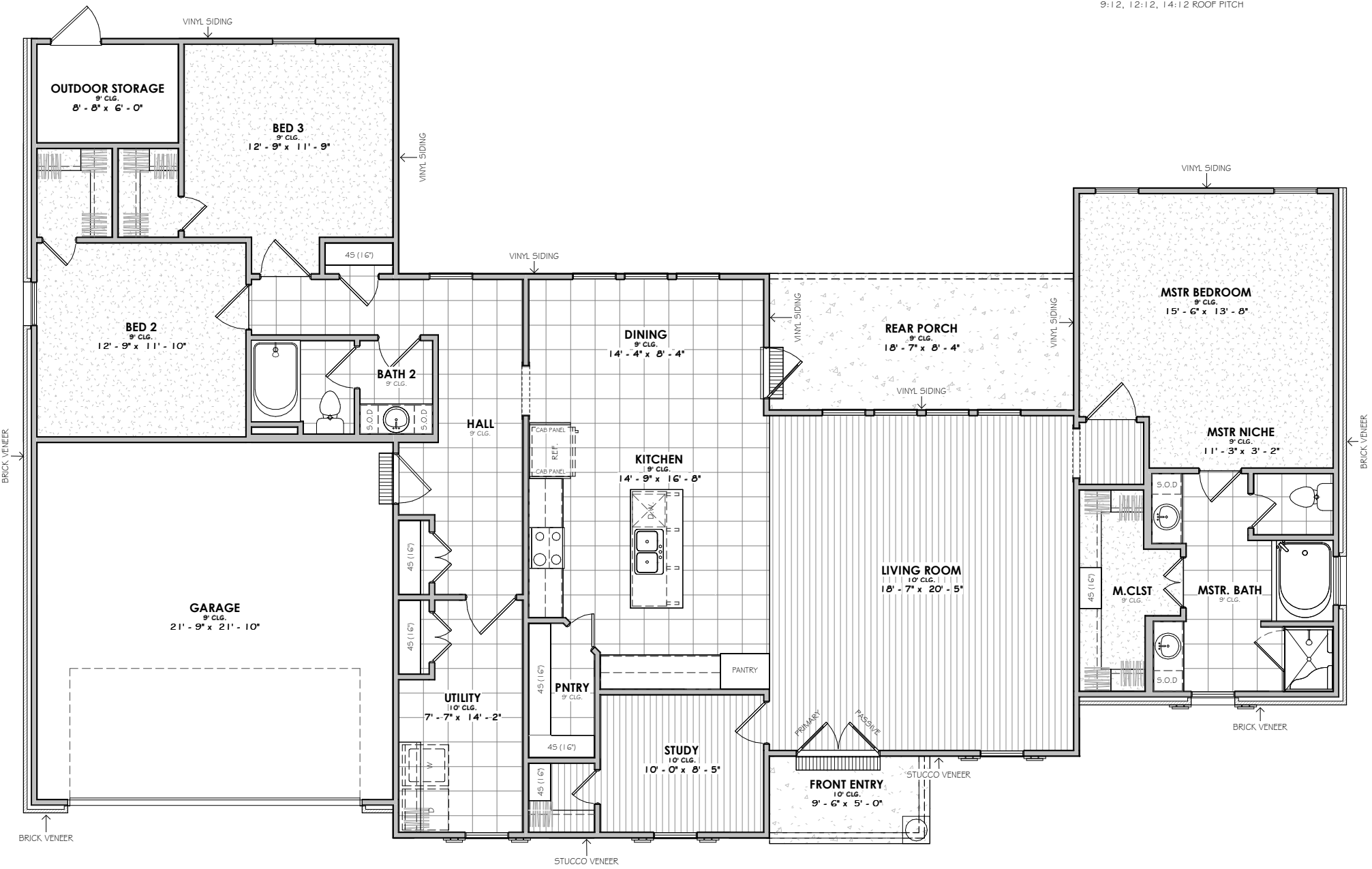
FLOOR PLAN
